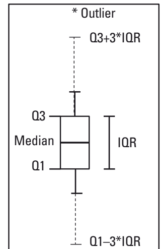
Figure 2: Outlier test according to 3*IQR boxplot method.
