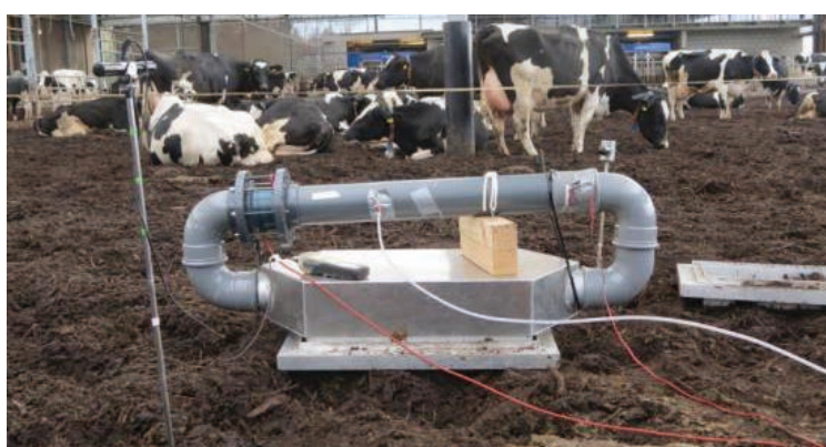
Figure 18: Closed flux chamber with air recirculation to measure the CO 2 production from bedding materials.
