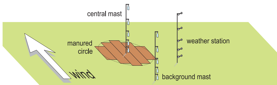
Figure 1. Layout of a circular plot for the measurement of NH 3 volatilization using the micrometeorological mass balance method, with masts supporting NH 3 traps at various heights in the centre of the plot and at the windward boundary of the plot.
